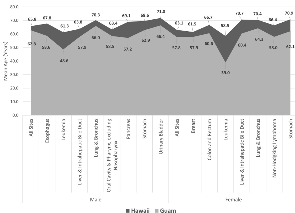
Fig. 3. Younger Age of Cancer Diagnosis ( p < 0.05 ) in Guam vs. Hawaii.
